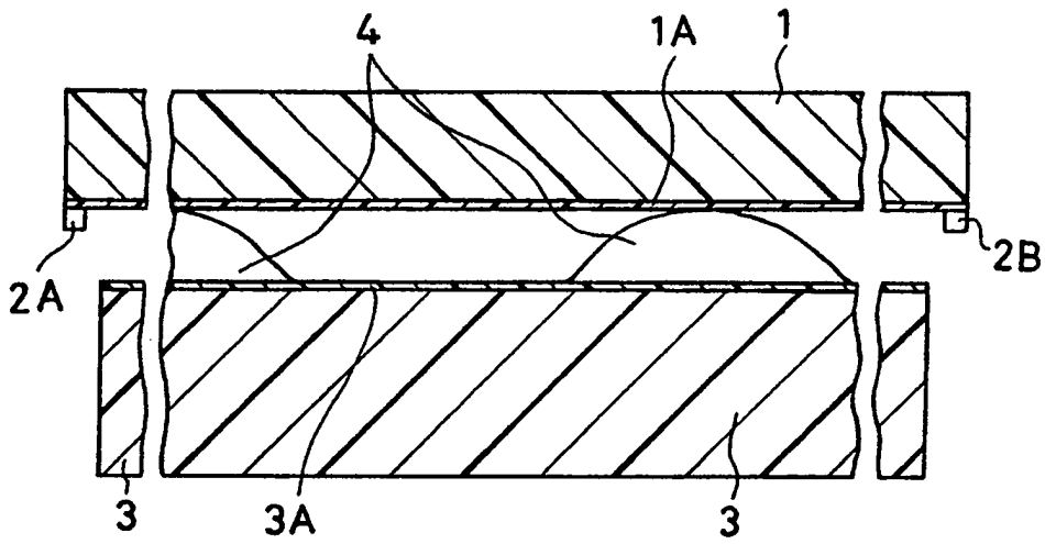
FIG.10 (Prior Art)
